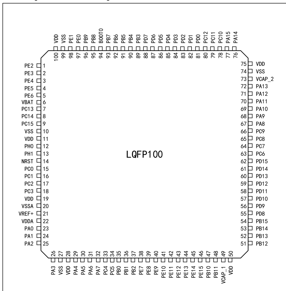
Figure 2 Distribution Diagram of APM32A407xGT7 Series LQFP100 Pins
